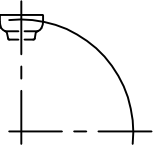
S.G. CPLING
